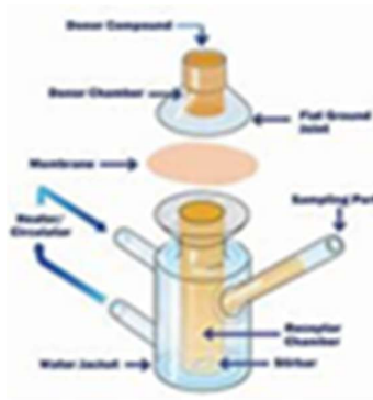
Figure 1. Franz diffusion cell device
